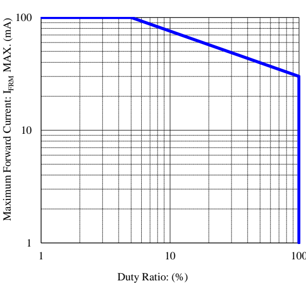
Duty Ratio vs. Maximum Forward Current
