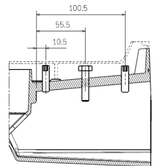
Section : Housing Bolt / Screw Layout
