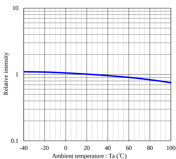
Relative intensity vs. Ambient temp.
