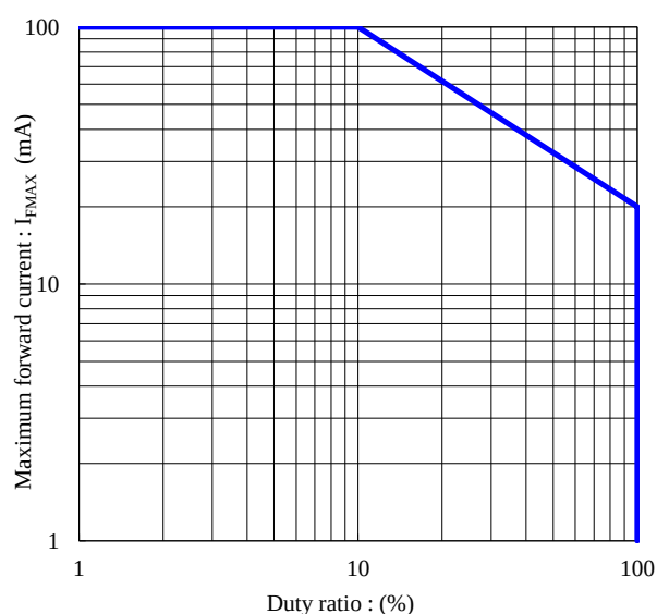
Max. forward current vs. Duty cycle
