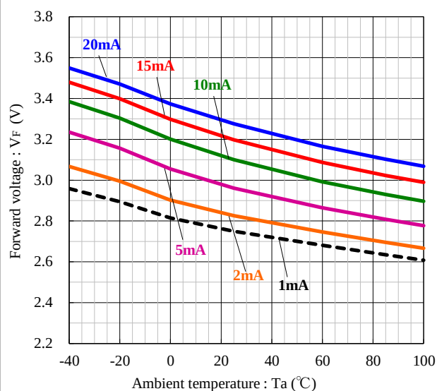
Forward voltage vs. Ambient temp.
