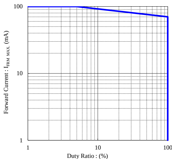
Maximum Forward Current vs. Duty Cycle
