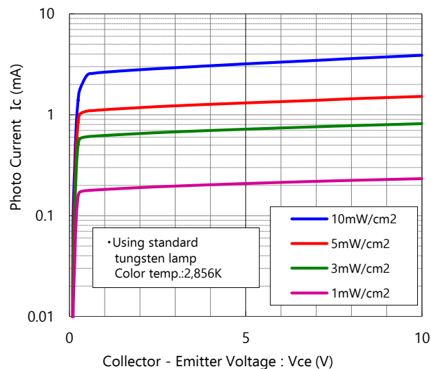
Collector-Emitter Voltage vs. Photo Current Condition: T_a=25^\circ C
