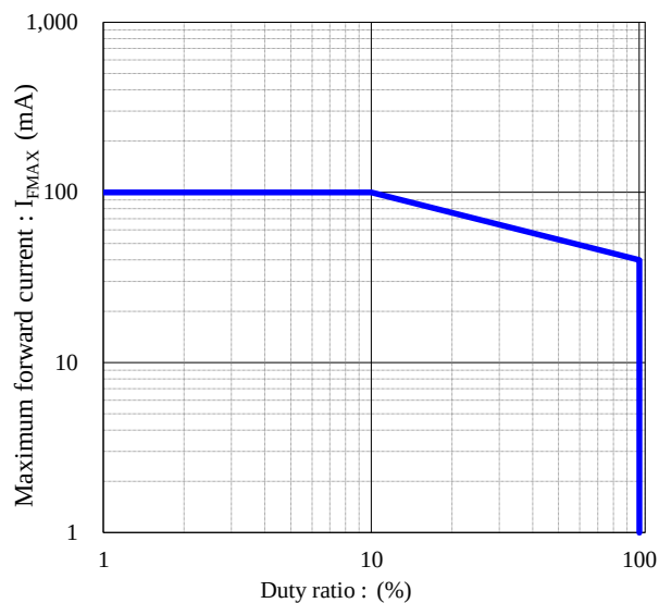
Max. forward current vs. Duty ratio
